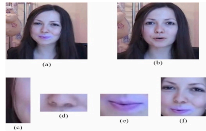
Fig. 4. Deepfake artifacts [89].
