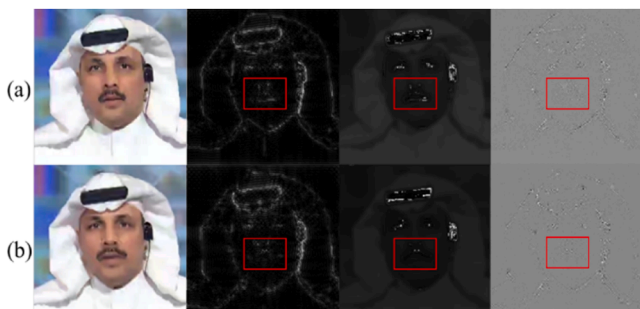
Fig. 5. Deepfake artifacts.
