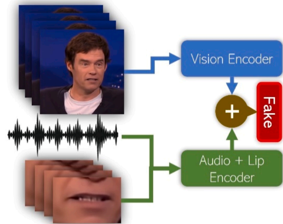
Fig. 6. Audio-visual synchronization.
